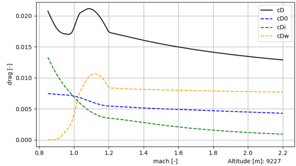
FIGURE 5: Drag vs. Mach number of a Concorde similar aircraft
